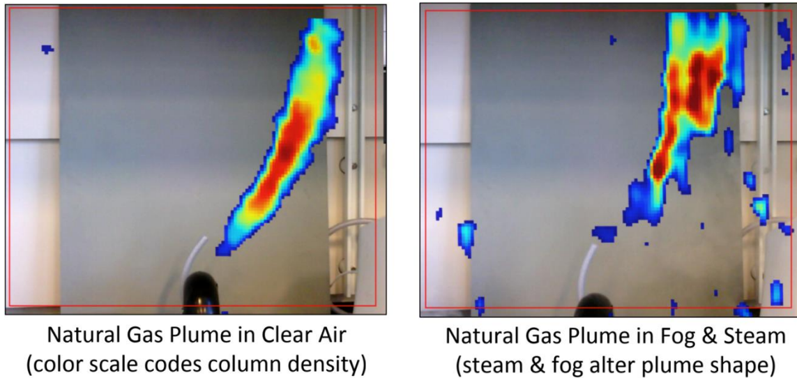
Figure 8 - Natural Gas Low Pressure Releases in Fumehood with and without Steam Addition at SAIT
